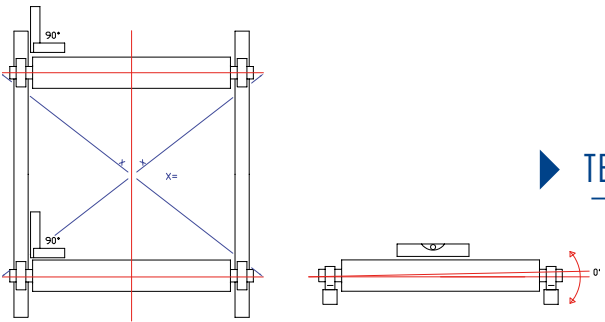
Geometry of the frame
