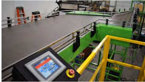
Inline High Speed Single Filer with Mass Accumulation Table
